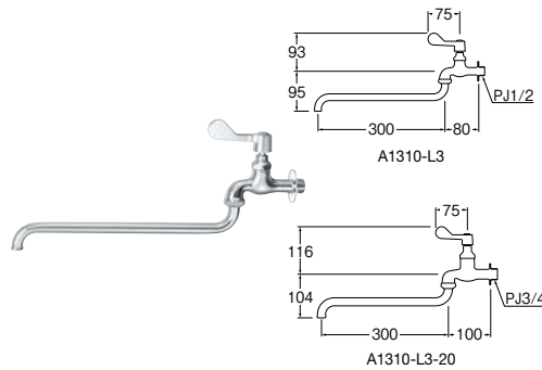
㊤ 厨房用自在水栓 [共用形]
