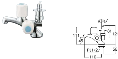
㊤洗濯機用二口立水栓
