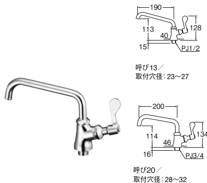
㊤ 厨房用立形上向自在水栓 [共用形]
