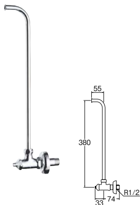
㊦ D式L管止水栓 [共用形]
