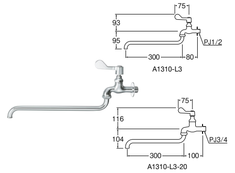
㊦ 厨房用自在水栓 [共用形]
