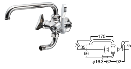
厨房用二口横形自在水栓 [共用形]
