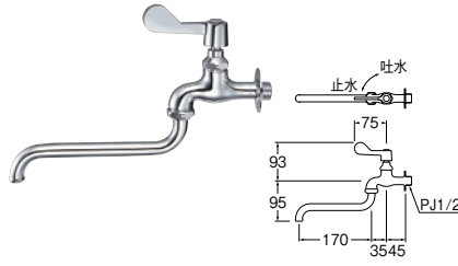
㊦ 厨房用自在水栓 [共用形]
