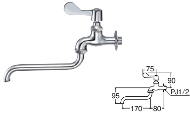
㊦ 厨房用自在水栓 [共用形]
